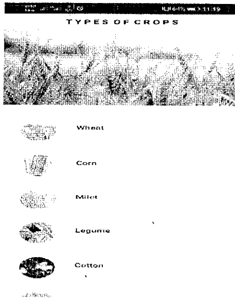
Fig7.5: Crop Screen
