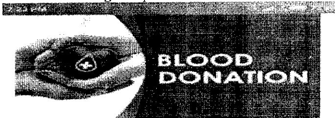
Fig7.1: Splash Screen
